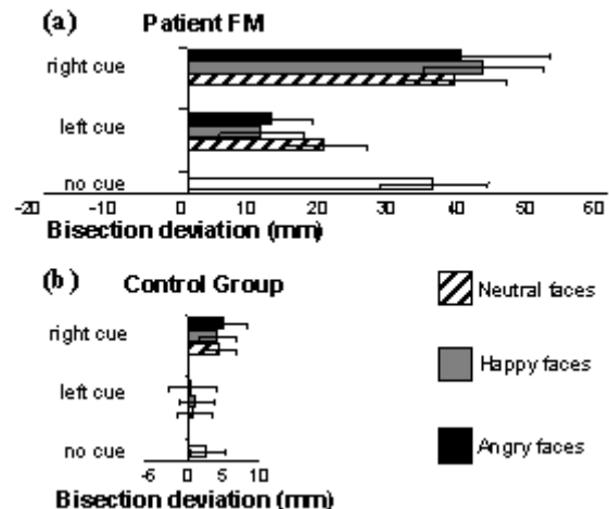
Figure 2: Mean error (mm) in the line bisection task for patient FM (a) and the Control Group (b) by cue position and cue type. Rightward errors are coded as positive, leftward as negative.
