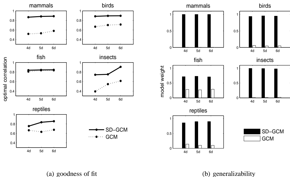
Figure 1: Optimal correlations between observed and model-based typicality scores (panel a) and model weights (panel b) for the GCM and the SD-GCM.
