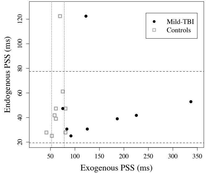
Figure 3. Exogenous (x-axis) and endogenous (y-axis) PSS scores in the TOJ task for each person with mild TBI and control participant. The area defined by the dotted vertical lines represents the 99% confidence interval for normal performance in the exogenous task based on the control data, and the area defined by the dotted horizontal lines similarly represents the 99% confidence intervals for the endogenous task.
