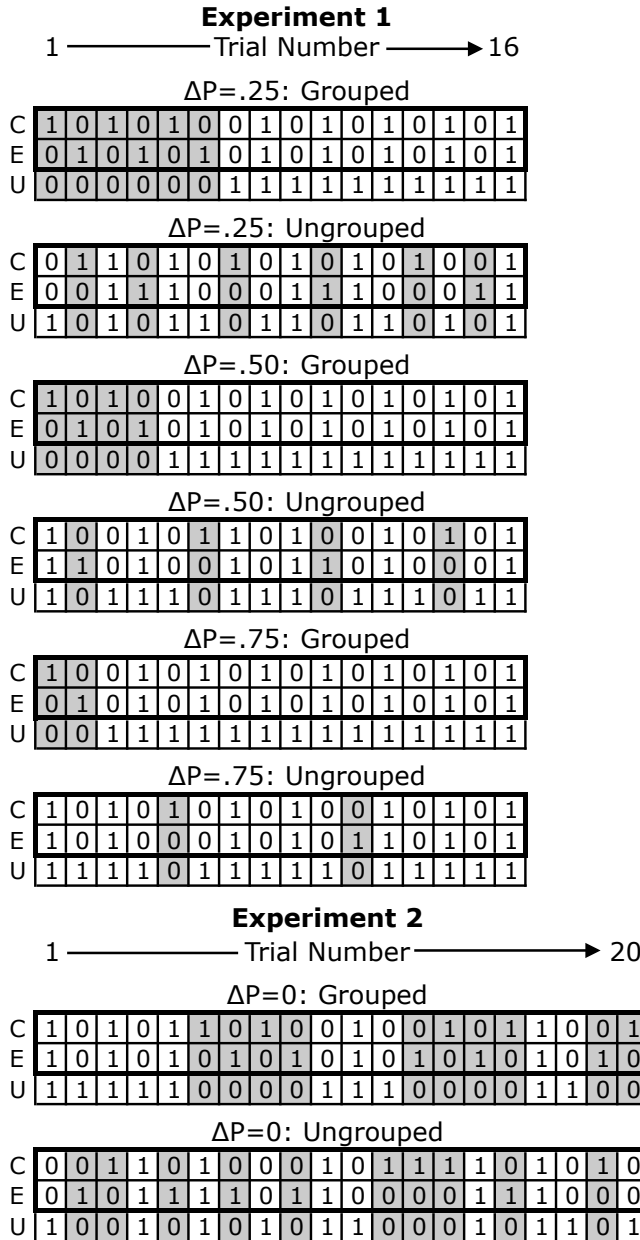
Figure 2: Summary of Stimuli in Experiments 1 and 2. Note: “U” represents an unobserved, interacting factor not shown to participants. Cells are gray when U=0.
